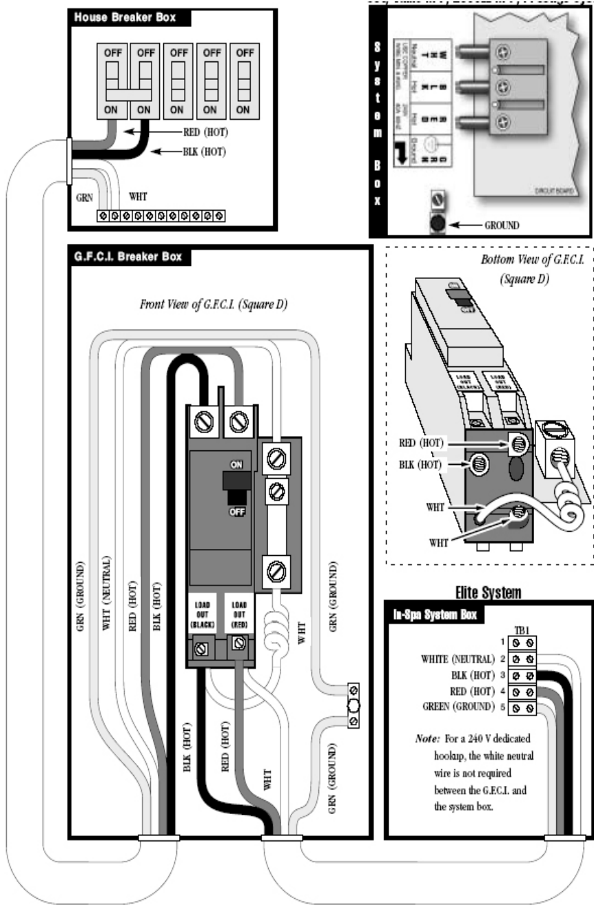
Electrical Wiring Diagram
